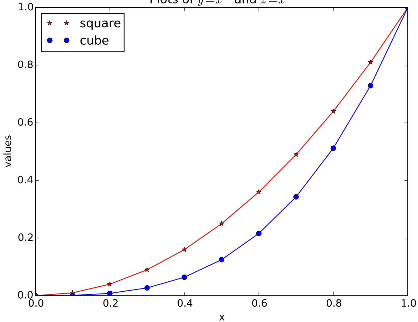
Plots of y=x^2 and z=x^3
